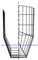
Provisional unfaired linesplan
