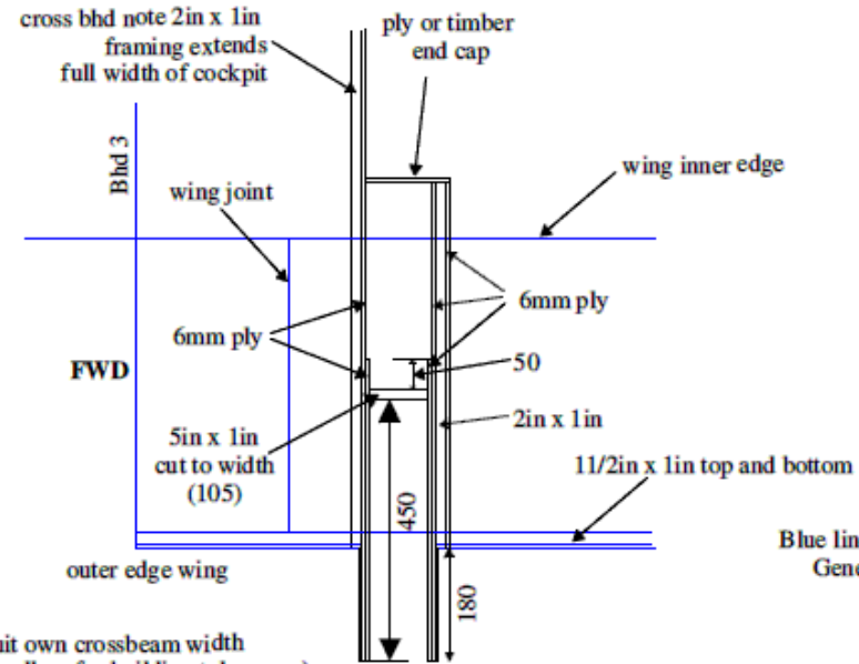
top view port box at pivot bolt
