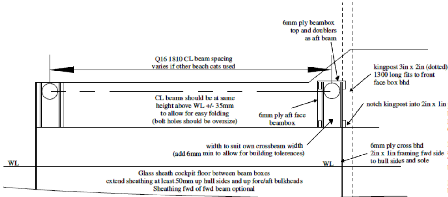
side view through beam boxes
