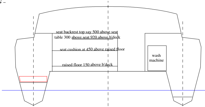
Cross Section at fwd saloon
